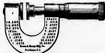
B. & S. PAPER GAUGE MICROMETER, No. 70
